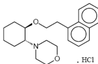
Figure 1: Chemical structure of RSD1070.
